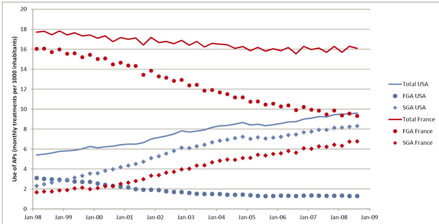
Figure 1. Trends in total antipsychotic, FGA and SGA use in the USA and in France
