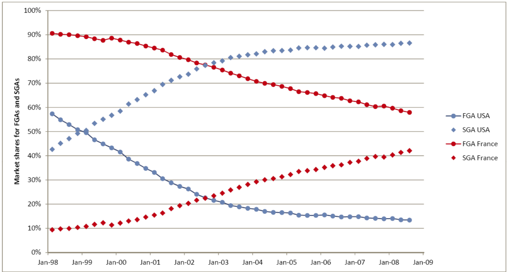
Figure 2. Evolution of FGA and SGA market shares in the USA and in France
